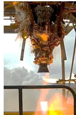
2013 BE-3 Engine Testing
